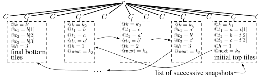
FIG. 5. Encoding of a TPG-CT instance in the proof of Theorem 5.6, with n = 3 (the number of tiles in a row).
