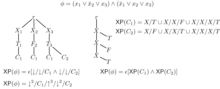
FIG. 1. Example encoding of a 3SAT instance \phi in the proofs of Propositions 4.2 and 4.3. Left: an XML tree conforming to the DTD defined in the reduction for \mathcal{X}(\downarrow, []) and \mathcal{X}(\downarrow, \uparrow) . Right: reduction for \mathcal{X}(\cup, []) .
